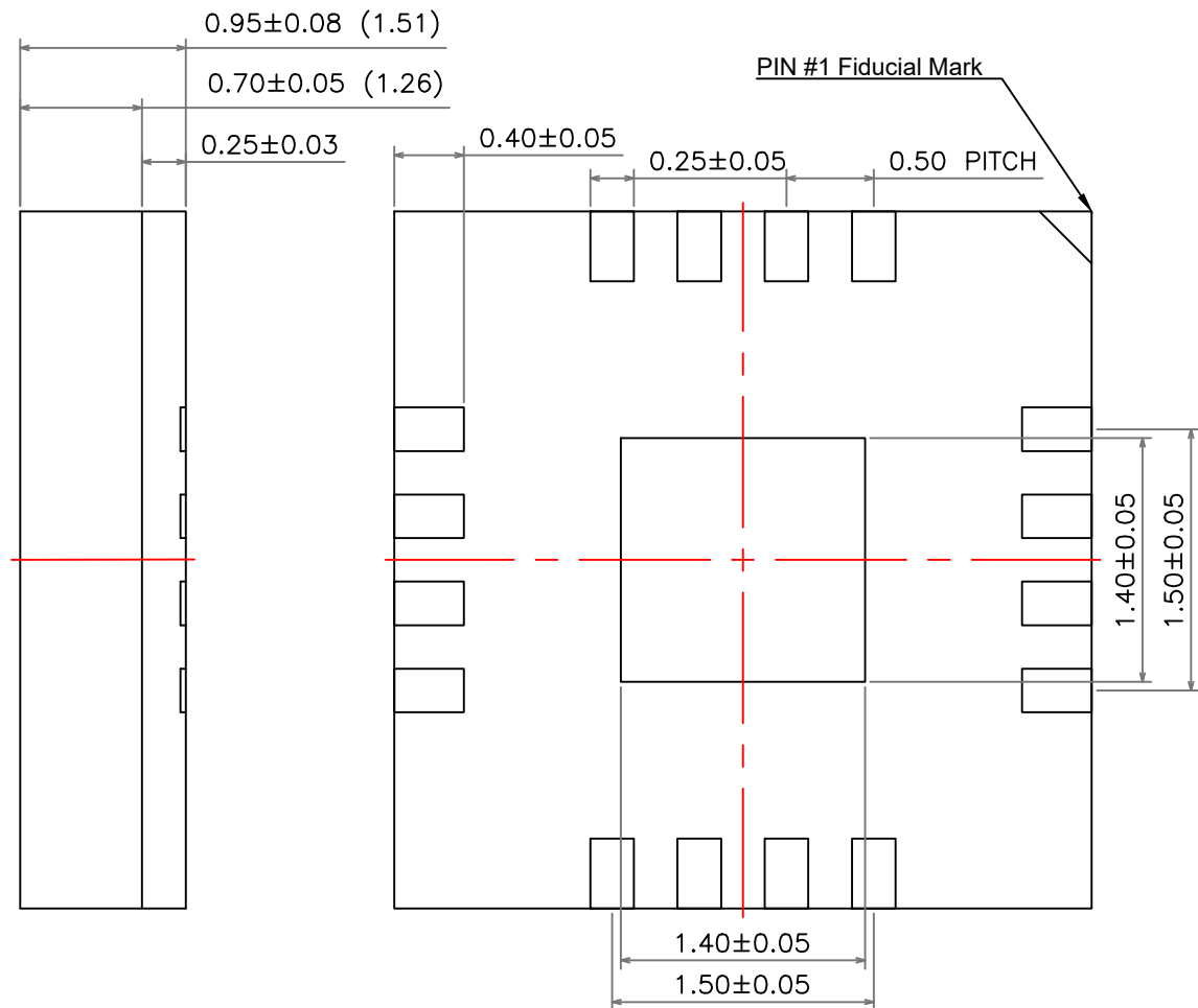
SIDE VIEW
